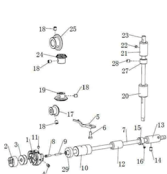
5. 勾线分组件 HOOK OF DRIVING SHAFT COMPONENTS
