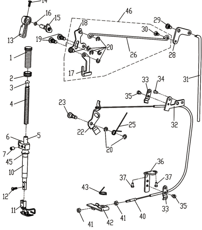
4. 压料、松线分组件 PRESSER BAR & TENSION RELEASE COMPONENTS
