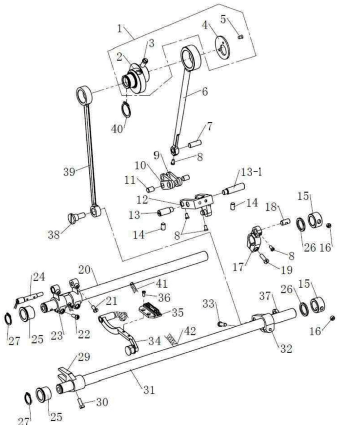
6. 送料分组件 FEED MECHANISM COMPONENTS
