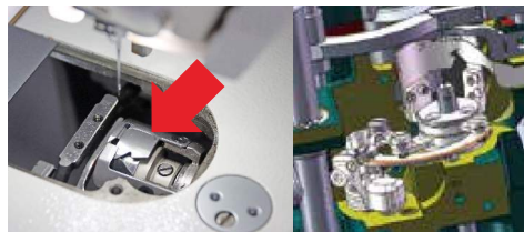
双刀智剪技术 Dual Blade Smart Cutting Technology
