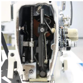
8420TD头部微油 8420DP The head of micro oil
