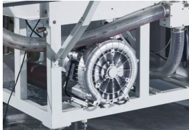
配备大功率高压旋涡风机，吸风效果强，噪音低 噪声低隔断式吸风装置箱，灵活切换进行吸附面料的工作 Equipped with High Power and Pressure Swirl Air Blower, Strong Sucking Effect, Low Noise, Partitioned Sucking Device Box, Flexible Switching for Suction of Fabrics.
