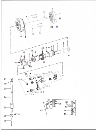
2. 针杆、压线部件 Needle bar and thread take-up mechanism
