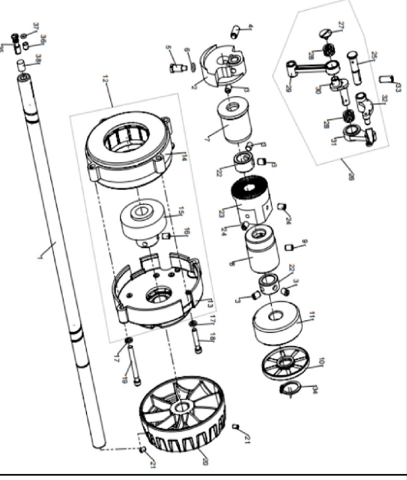
2. 主轴、换线分组件 MAIN SHAFT & THREAD TAKE-UP COMPONENTS
