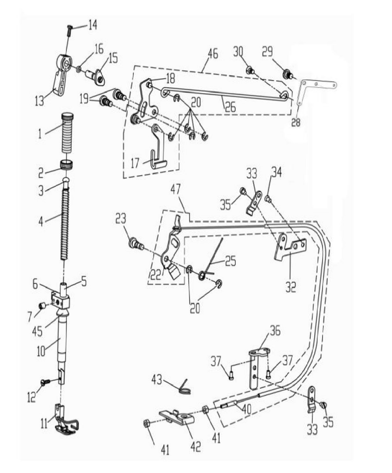
4. 压料、松线分组件 PRESSER BAR & TENSION RELEASE COMPONENTS
