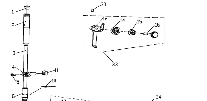
3. 针杆、夹线分组件 NEEDLE BAR & THREAD TENSION COMPONENTS
