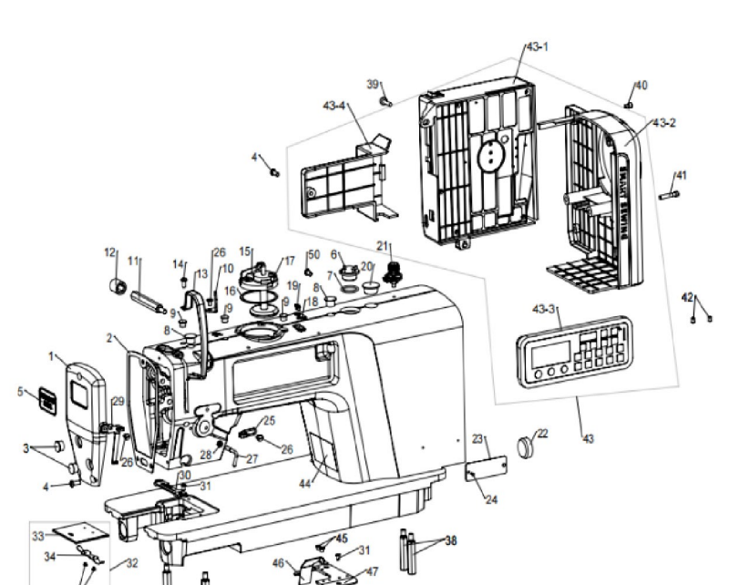
1. 机壳分组件 MACHINE FRAMMISCELLANEOUS COVER COMPONENTS
