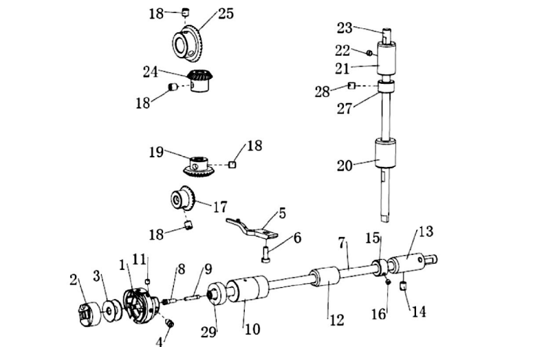
5. 勾线分组件 HOOK OF DRIVING SHAFT COMPONENTS
