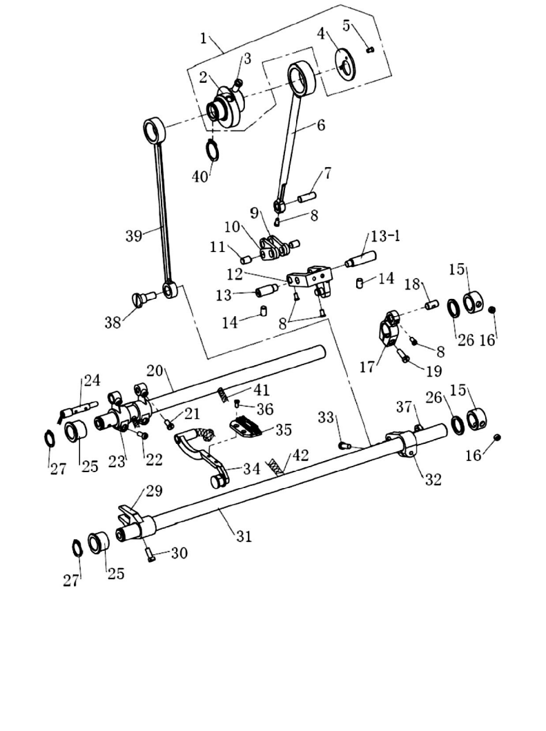
6. 送料分组件 FEED MECHANISM COMPONENTS
