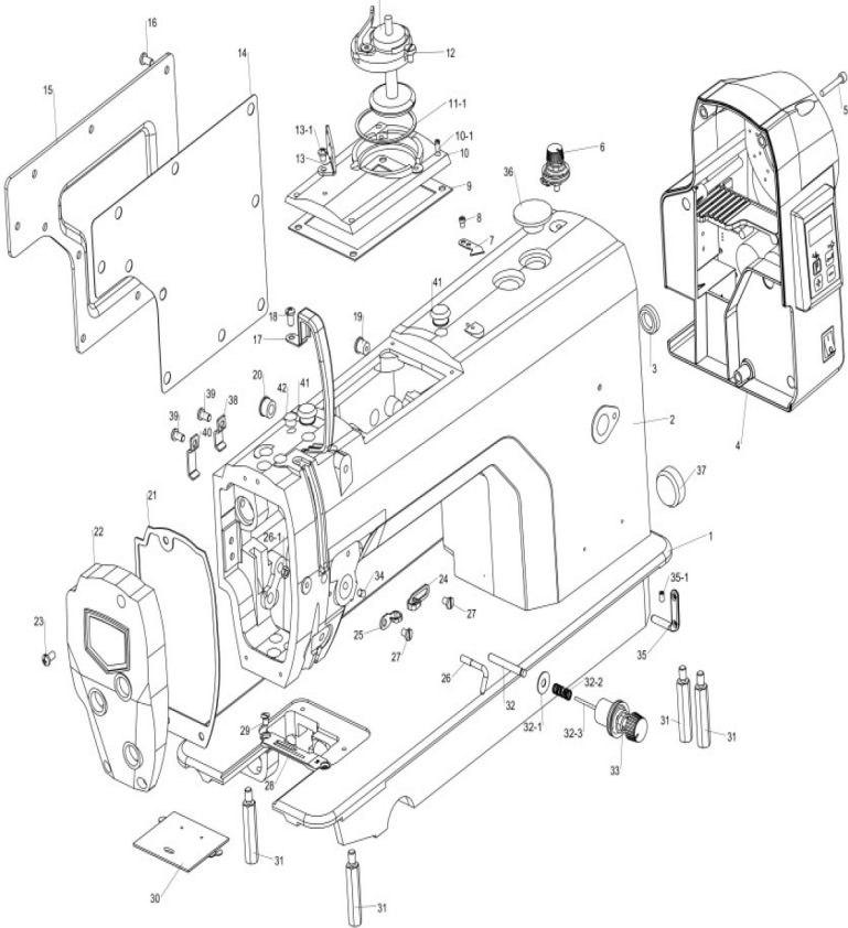
1. 机体部件 / MACHINE MECHANISM
