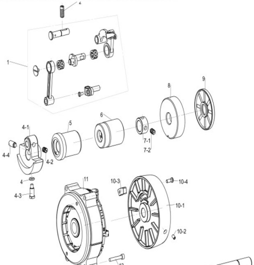
2. 上轴、换线装置 / MAIN SHAFT/THREAD-UP LEVER MECHANISM
