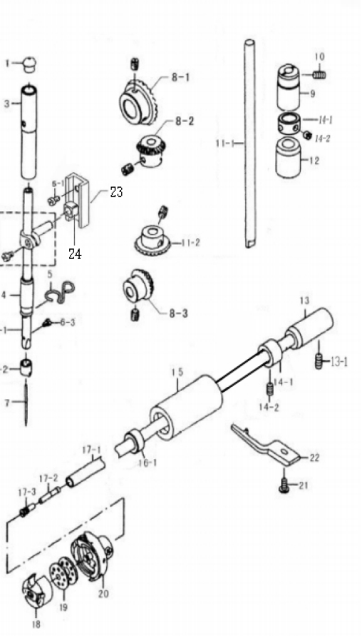
3. 针杆、竖轴、下轴装置 / NEEDLE BAR UPRIGHT SHAFT/SHOULDER DRIVING SHAFT MECHANISM
