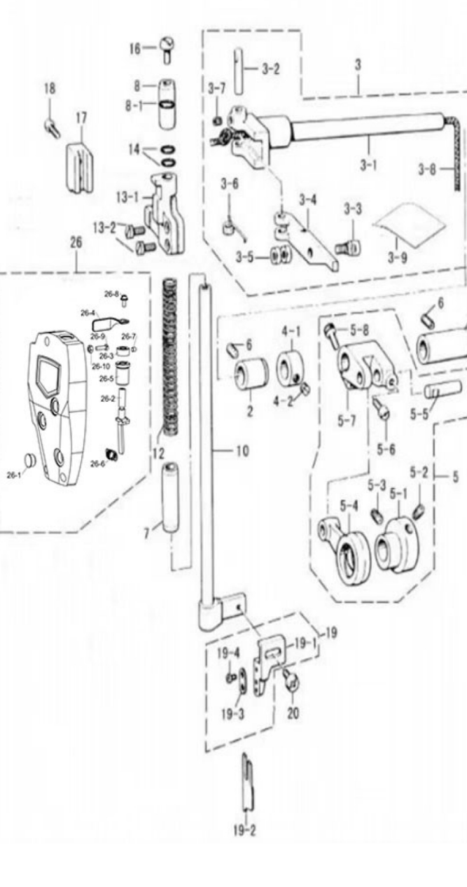
6. 切刀部件 / UPPER KNIFE MECHANISM
