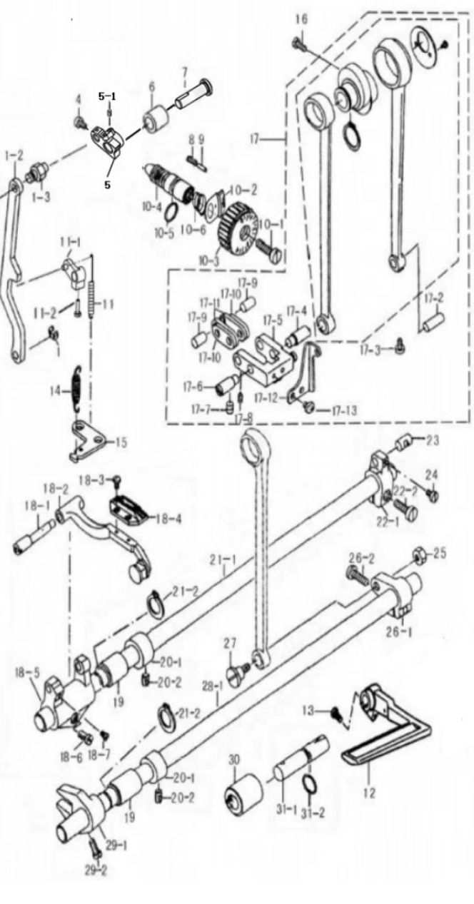
5. 送料装置 / FEED MECHANISM
