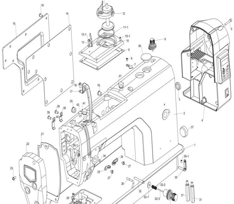
1. 机体部件 / MACHINE MECHANISM
