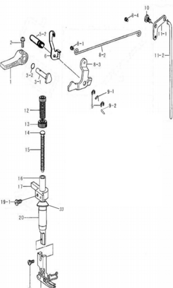
4. 压脚装置 / PRESSER FOOT MECHANISM
