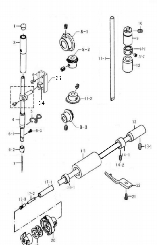
3. 针杆、竖轴 / NEEDLE BAR UPRIGHT SHAFT/ROCK DRIVING SHAFT MECHANISM
