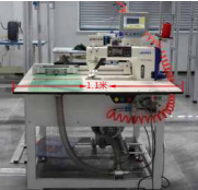
窄幅面台板，空间小，适应各种吊挂线。 Narrow surface platform, small space, suitable for a variety of hanging stations
