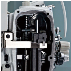
头部微油 The head of micro oil
