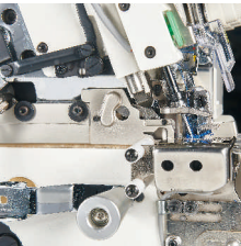
侧吸剪线刀机构(选配) side suction thread trimmer mechanism (optional)
