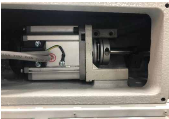
上下双伺服独立驱动, 高速、静音、低振; Up and down double servo independent drive, high speed, quiet, low vibration;
