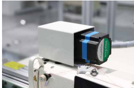
步进电机抬压脚，可实现中段控制，能适应不同面料。 step motor lift foot, can achieve the middle control, can adapt to different fabrics.
