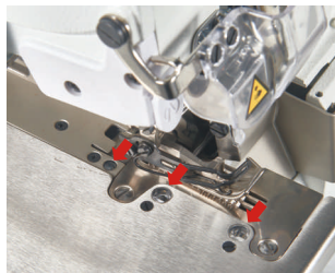
三光眼，防切布 Infrared light, prevent from cutting cloth
